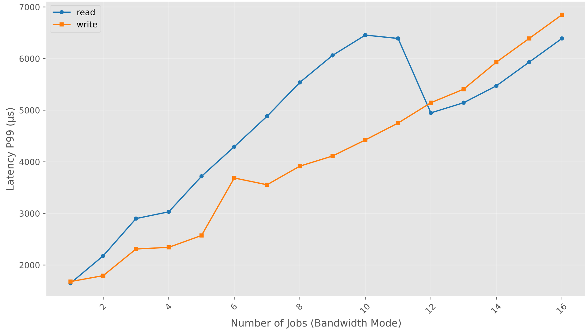
Latency P99 vs Number of Jobs (Bandwidth Mode)
